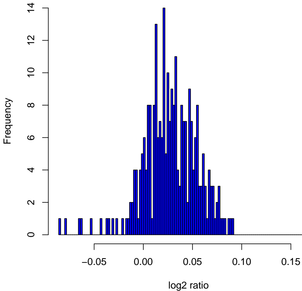
Histogram of log 2 ratios in 270 HapMap samples at clone Chr4tp-21C1
