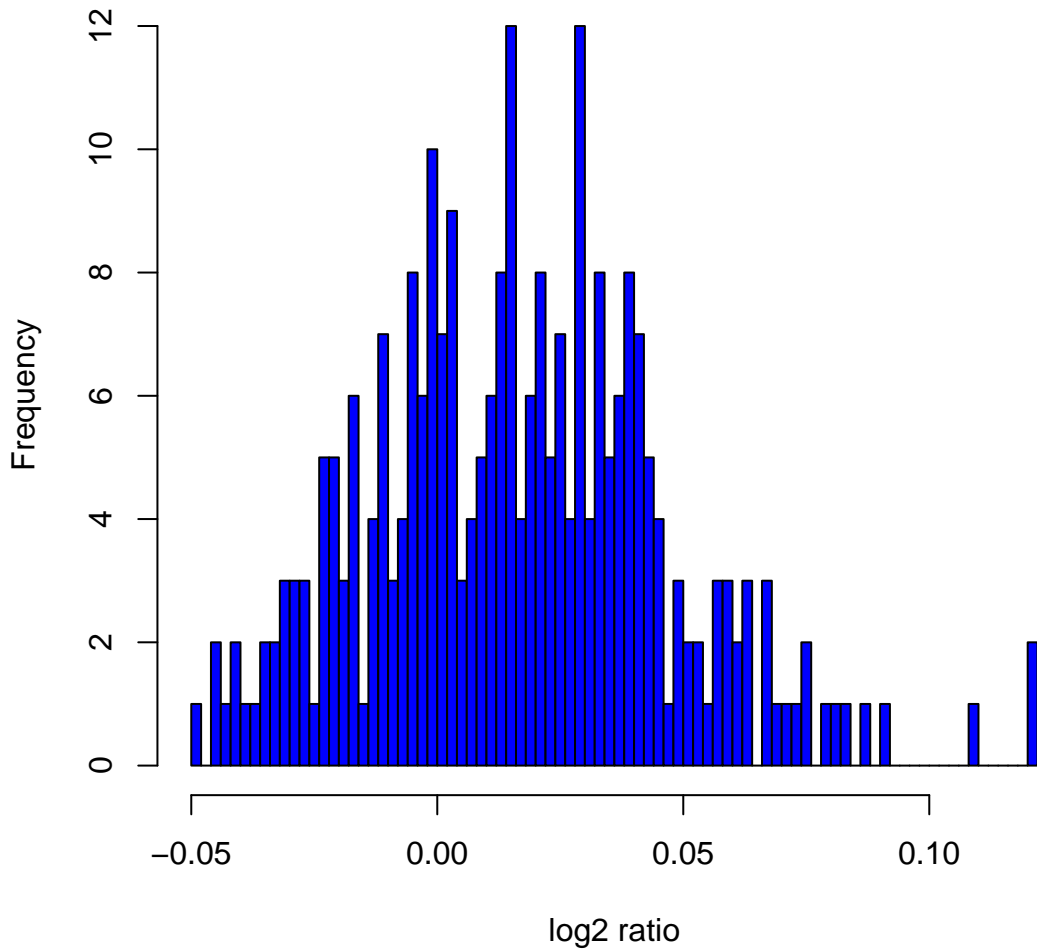
Histogram of \log_2 ratios in 270 HapMap samples at clone Chr4tp-21C5
