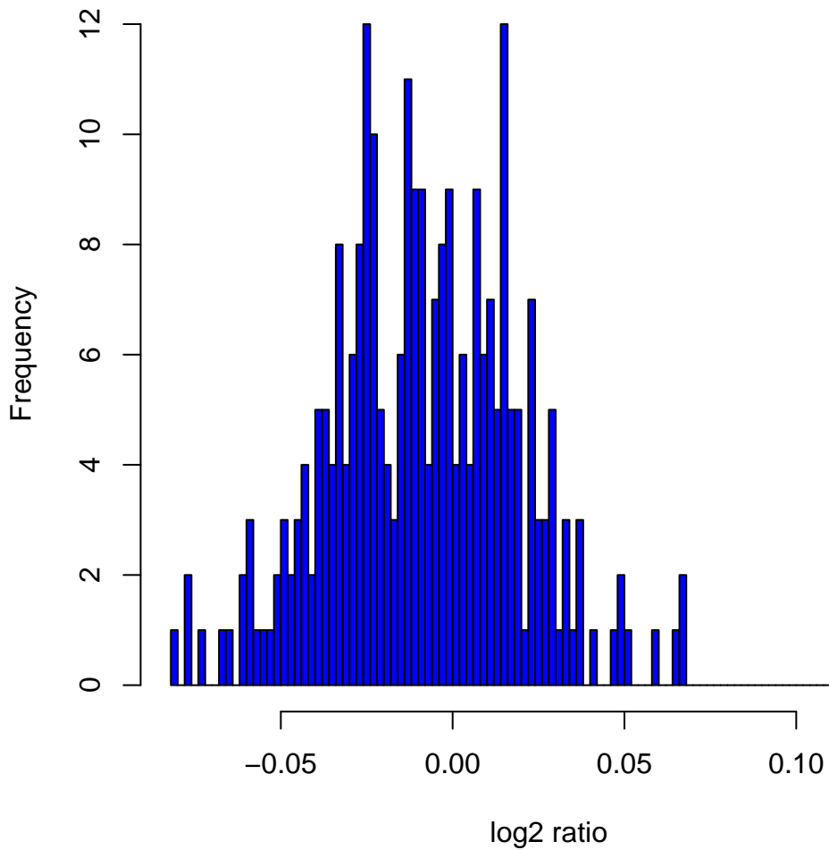
Histogram of log 2 ratios in 270 HapMap samples at clone Chr4tp-21C7
