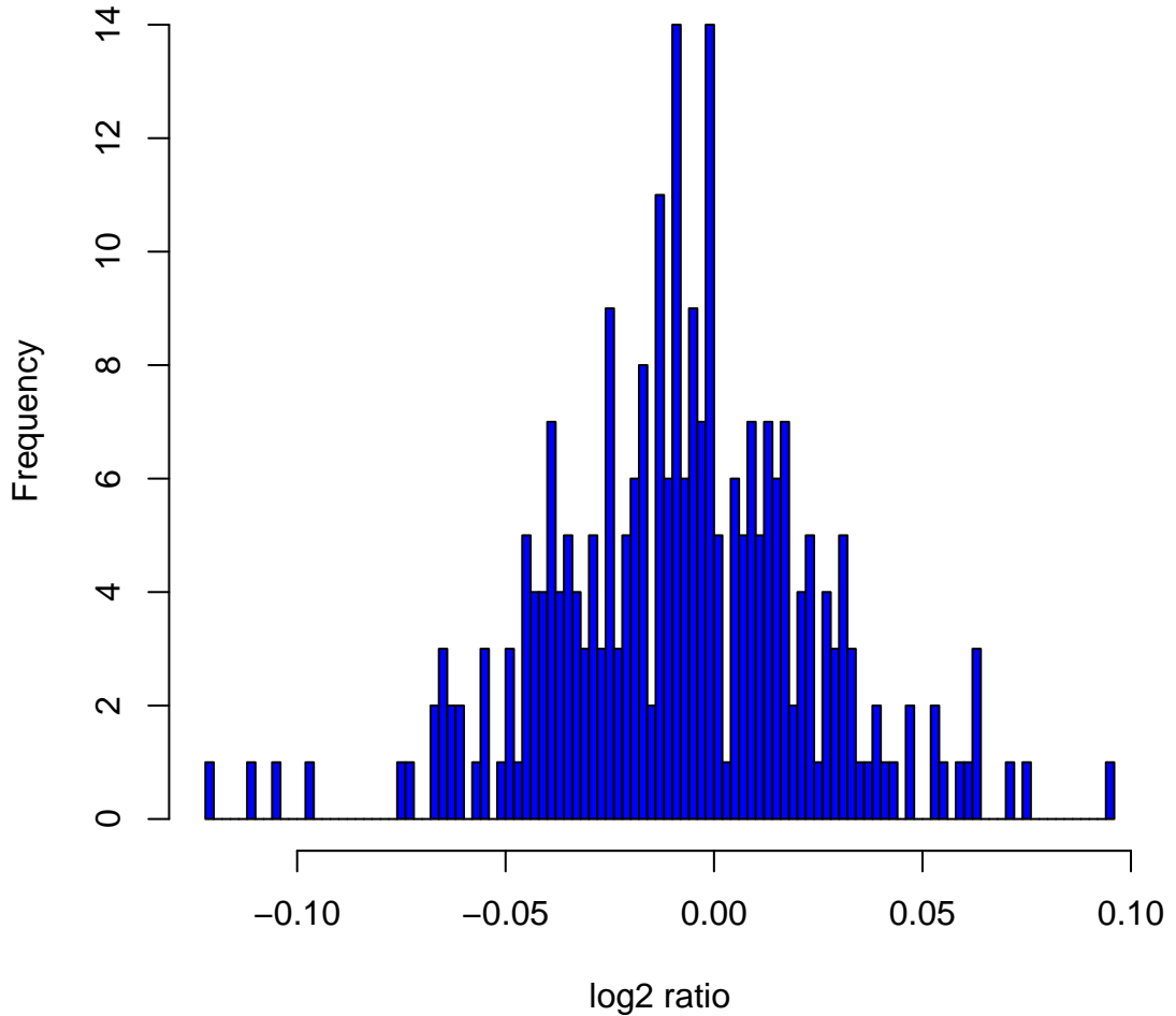
Histogram of log2ratios in 270 HapMap samples at clone Chr4tp-21D11
