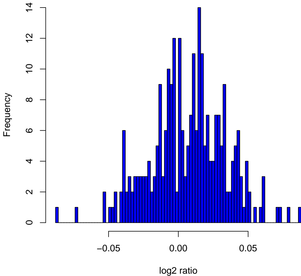
Histogram of log 2 ratios in 270 HapMap samples at clone Chr4tp-21F5
