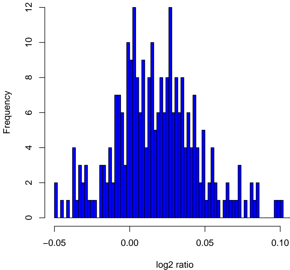
Histogram of \log_2 ratios in 270 HapMap samples at clone Chr4tp-21G1
