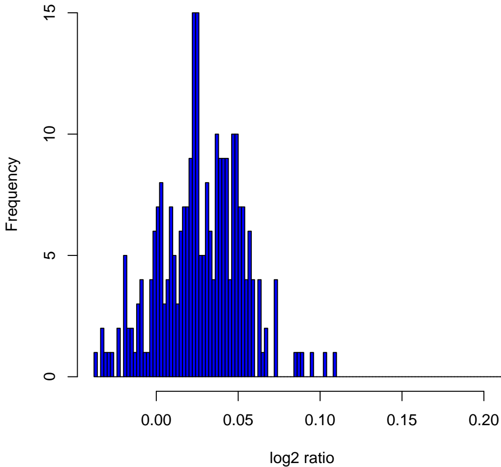
Histogram of log2ratios in 270 HapMap samples at clone Chr4tp-21G11
