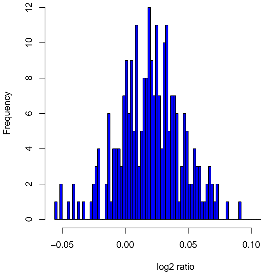
Histogram of \log_2 ratios in 270 HapMap samples at clone Chr4tp-21H11
