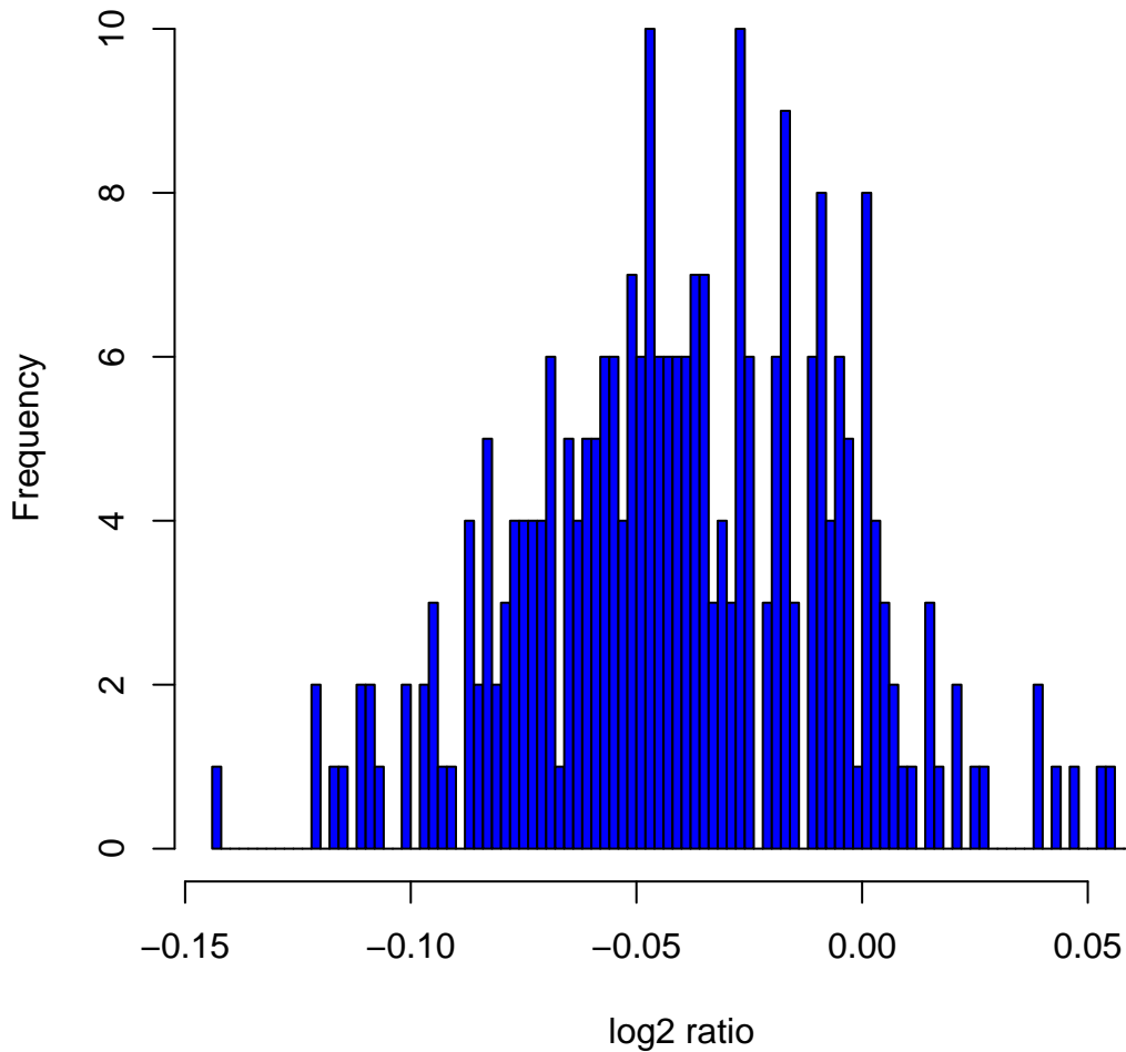
Histogram of log 2 ratios in 270 HapMap samples at clone Chr4tp-21H2
