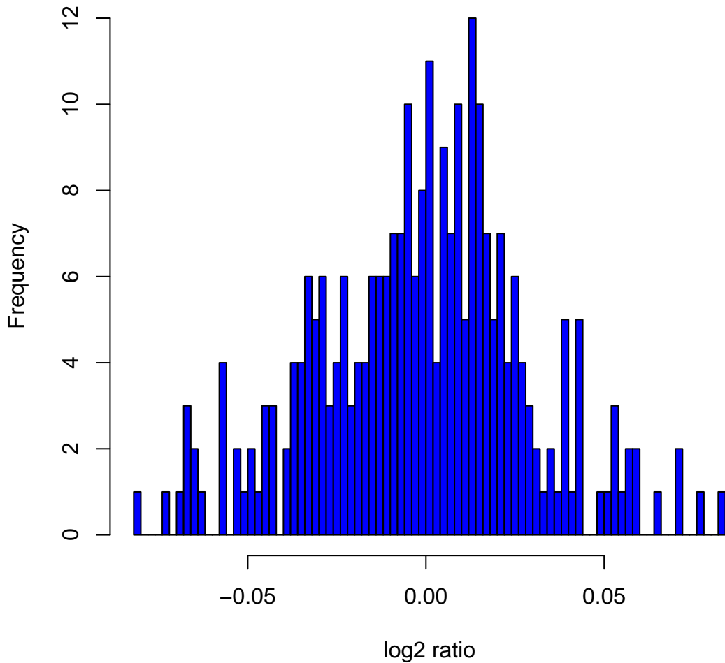
Histogram of log 2 ratios in 270 HapMap samples at clone Chr4tp-22C6
