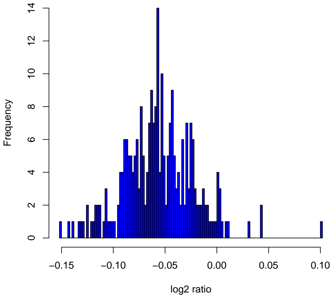
Histogram of log2ratios in 270 HapMap samples at clone Chr4tp-22D11
