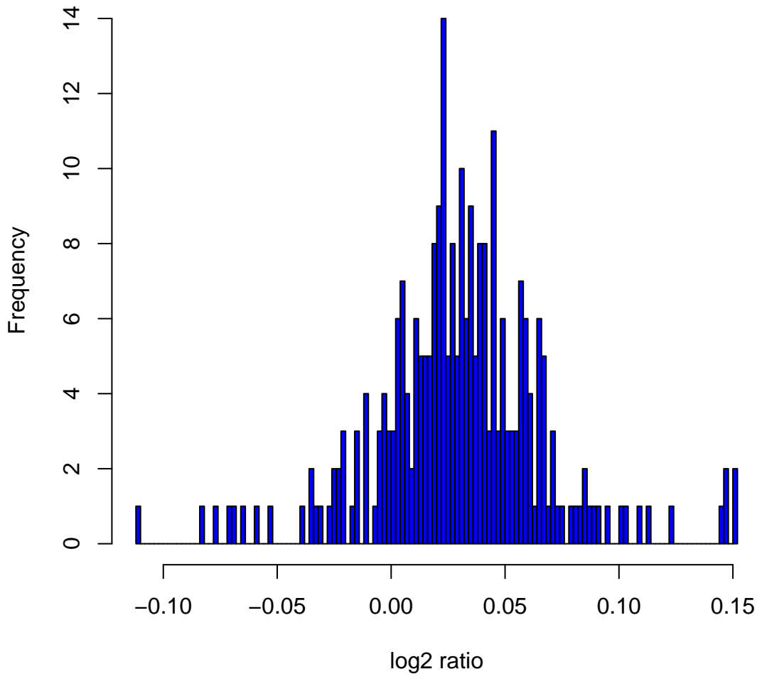
Histogram of log2ratios in 270 HapMap samples at clone Chr4tp-22E12
