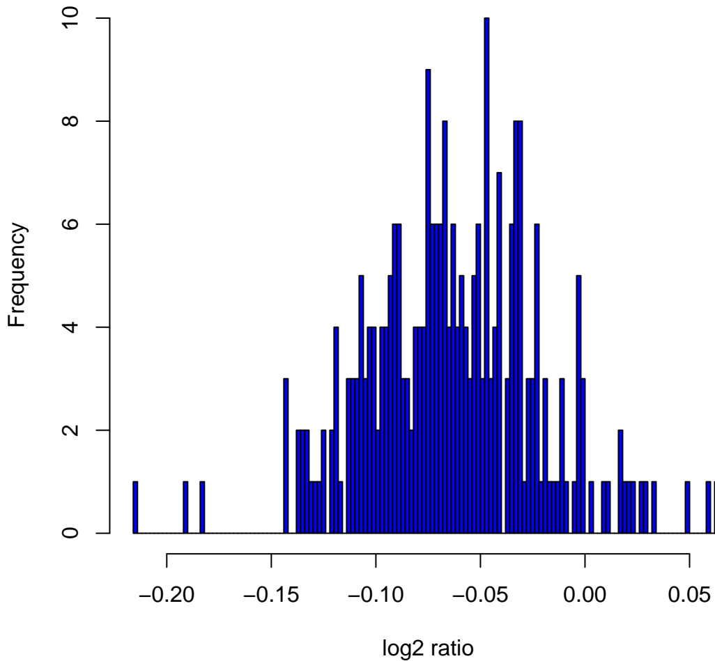
Histogram of log 2 ratios in 270 HapMap samples at clone Chr4tp-22G6
