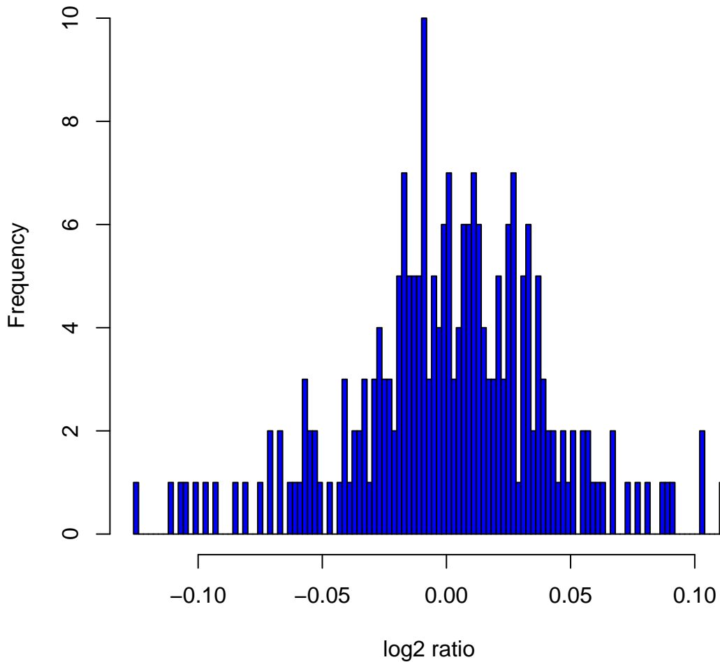
Histogram of log2ratios in 270 HapMap samples at clone Chr4tp-23B12
