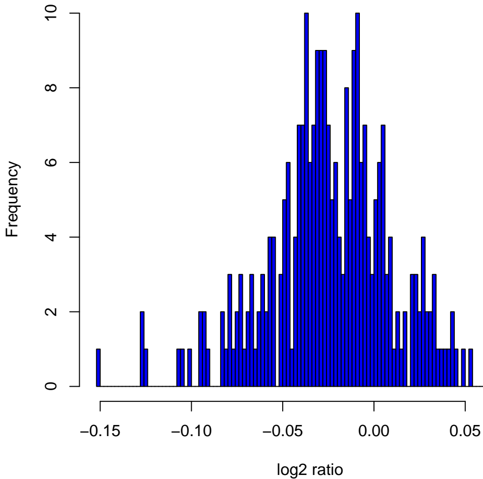
Histogram of log 2 ratios in 270 HapMap samples at clone Chr4tp-23B3
