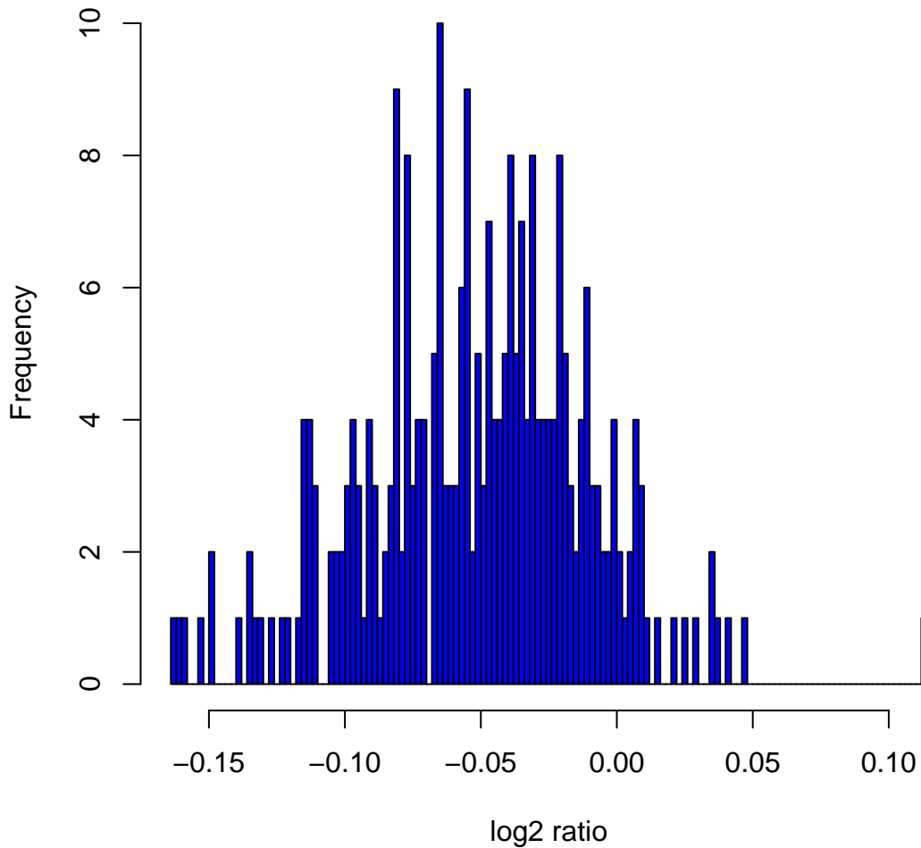
Histogram of \log_2 ratios in 270 HapMap samples at clone Chr4tp-23G1
