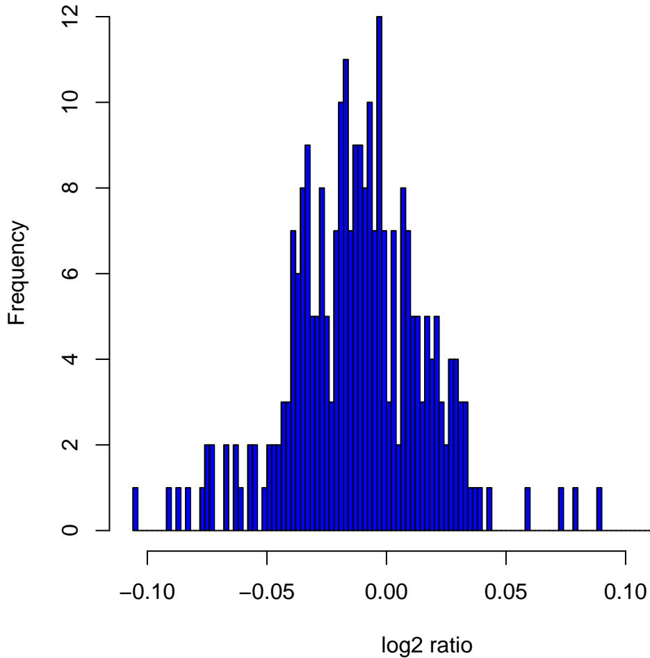
Histogram of log 2 ratios in 270 HapMap samples at clone Chr4tp-23G3
