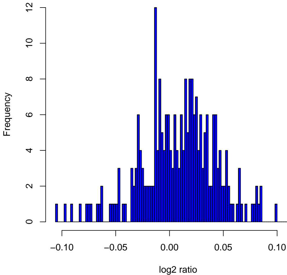
Histogram of log 2 ratios in 270 HapMap samples at clone Chr4tp-23G6
