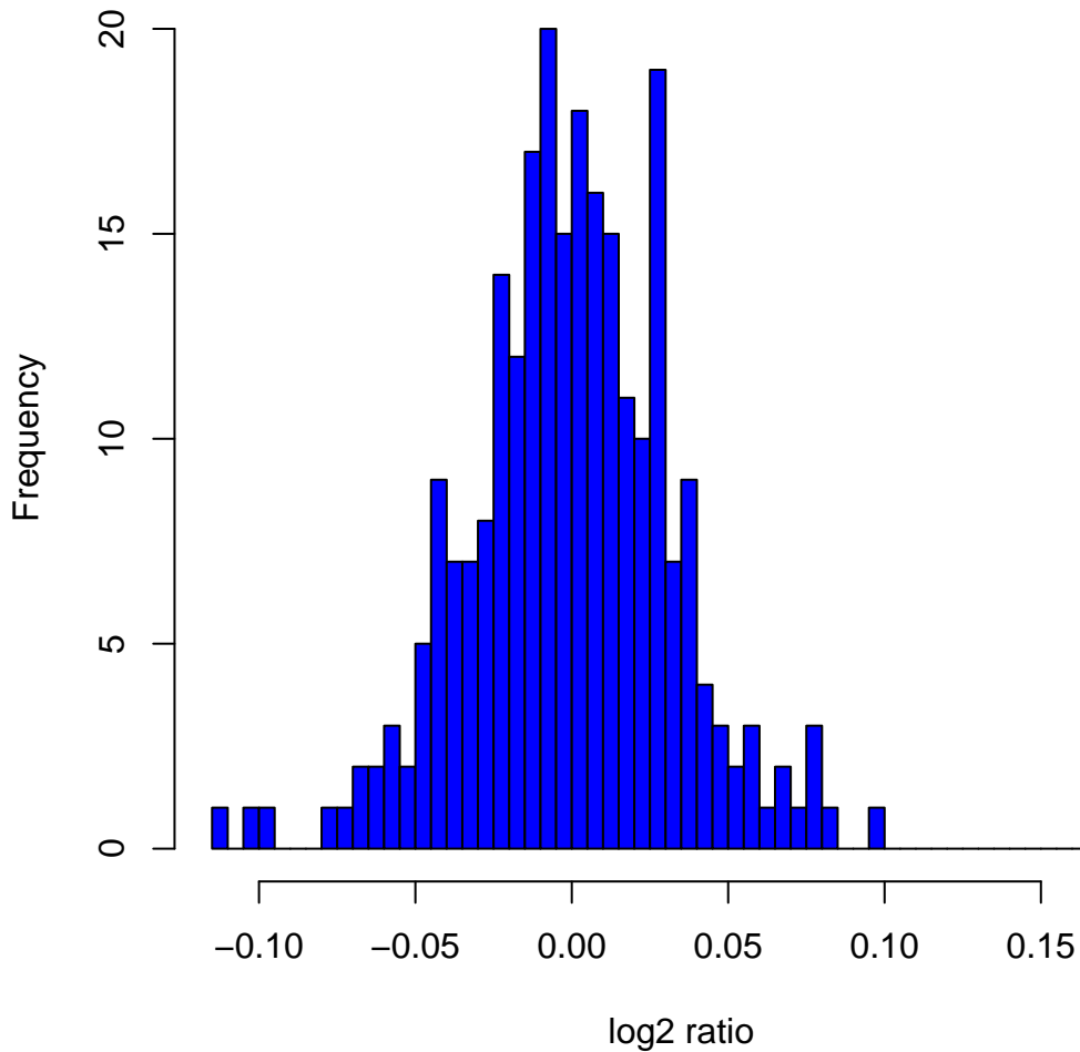
Histogram of \log_2 ratios in 270 HapMap samples at clone Chr4tp-24E12
