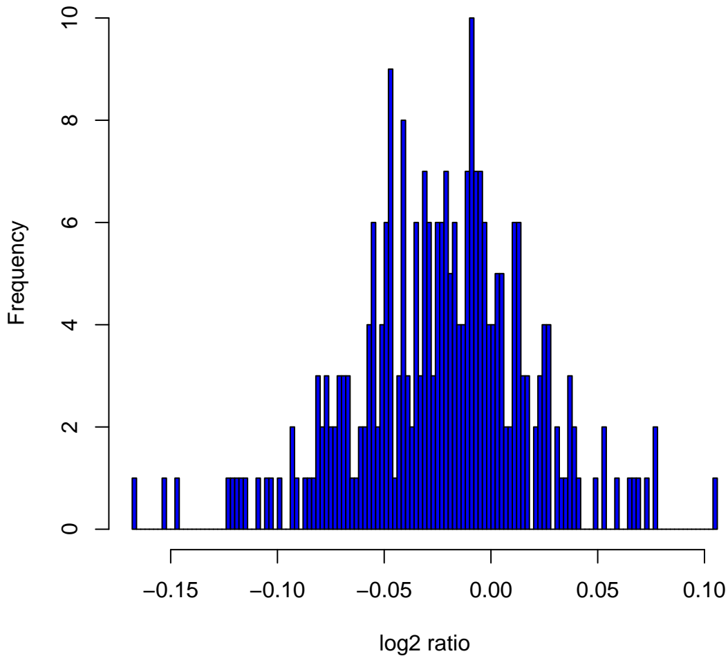
Histogram of log 2 ratios in 270 HapMap samples at clone Chr4tp-24G7
