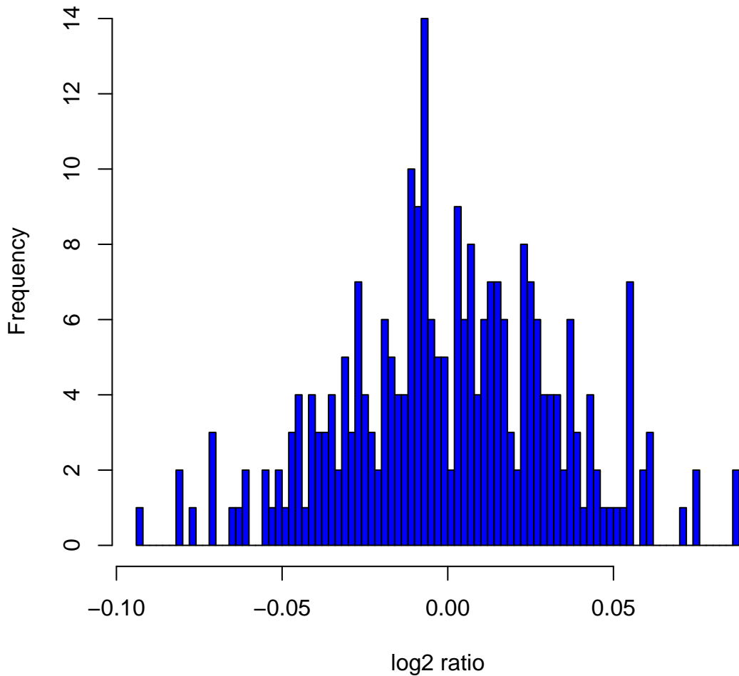
Histogram of log2ratios in 270 HapMap samples at clone Chr4tp-25B5
