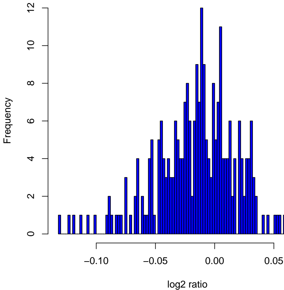
Histogram of log 2 ratios in 270 HapMap samples at clone Chr4tp-25B7
