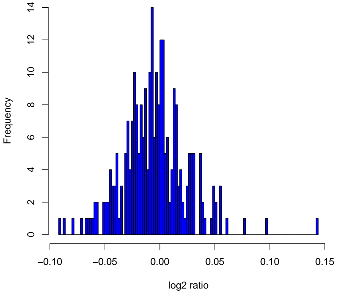
Histogram of log 2 ratios in 270 HapMap samples at clone Chr4tp-25D4
