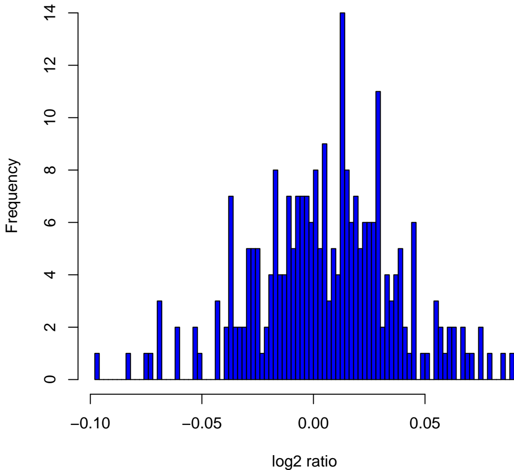
Histogram of log 2 ratios in 270 HapMap samples at clone Chr4tp-25D8
