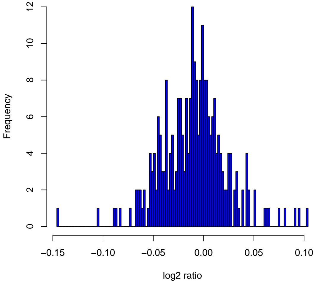
Histogram of log2ratios in 270 HapMap samples at clone Chr4tp-26A11
