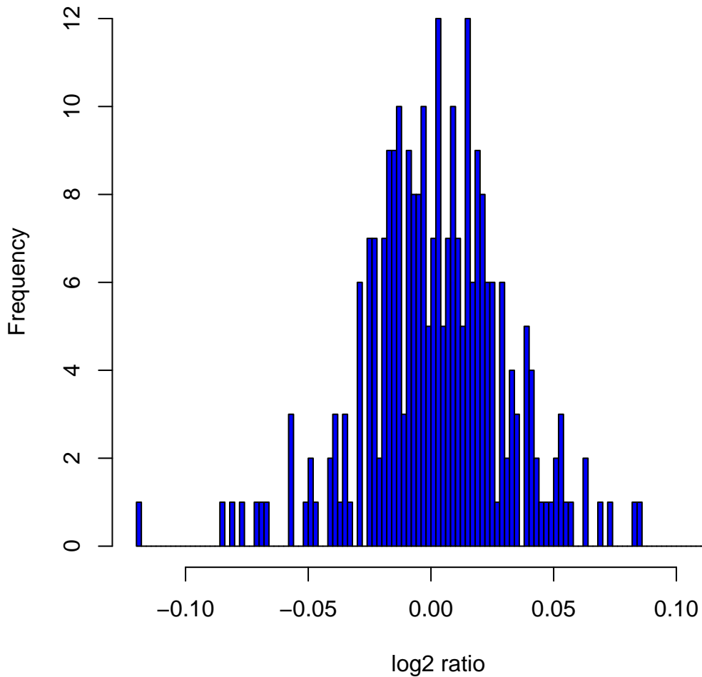
Histogram of log 2 ratios in 270 HapMap samples at clone Chr4tp-2A11
