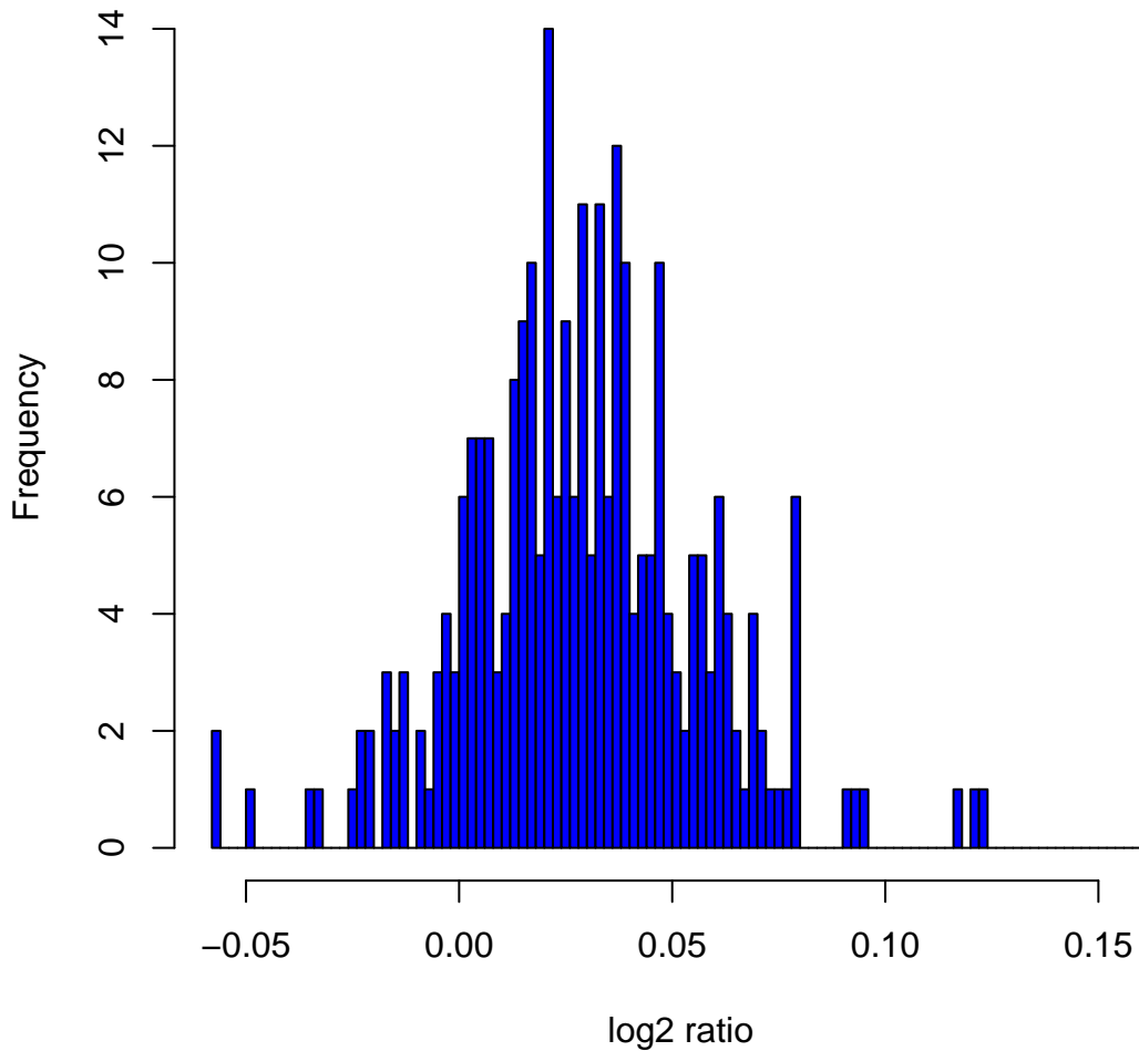
Histogram of log 2 ratios in 270 HapMap samples at clone Chr4tp-2A4
