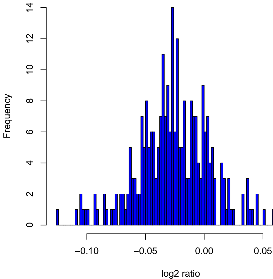
Histogram of log 2 ratios in 270 HapMap samples at clone Chr4tp-2A7
