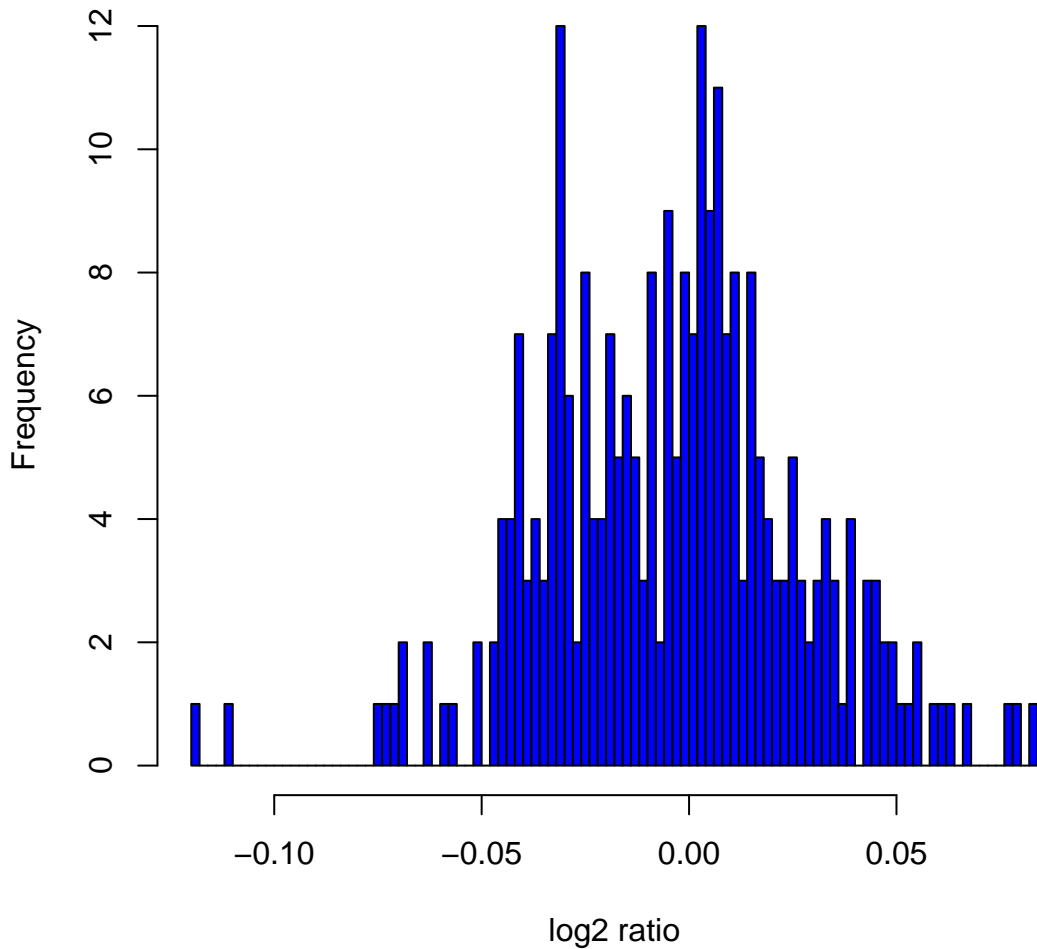
Histogram of log 2 ratios in 270 HapMap samples at clone Chr4tp-2A8
