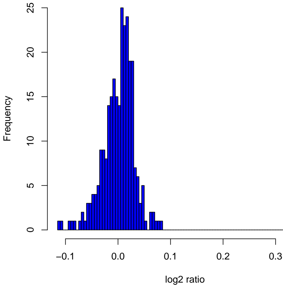
Histogram of \log_2 ratios in 270 HapMap samples at clone Chr4tp-2B10
