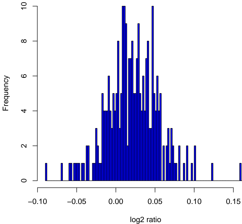
Histogram of \log_2 ratios in 270 HapMap samples at clone Chr4tp-2B3
