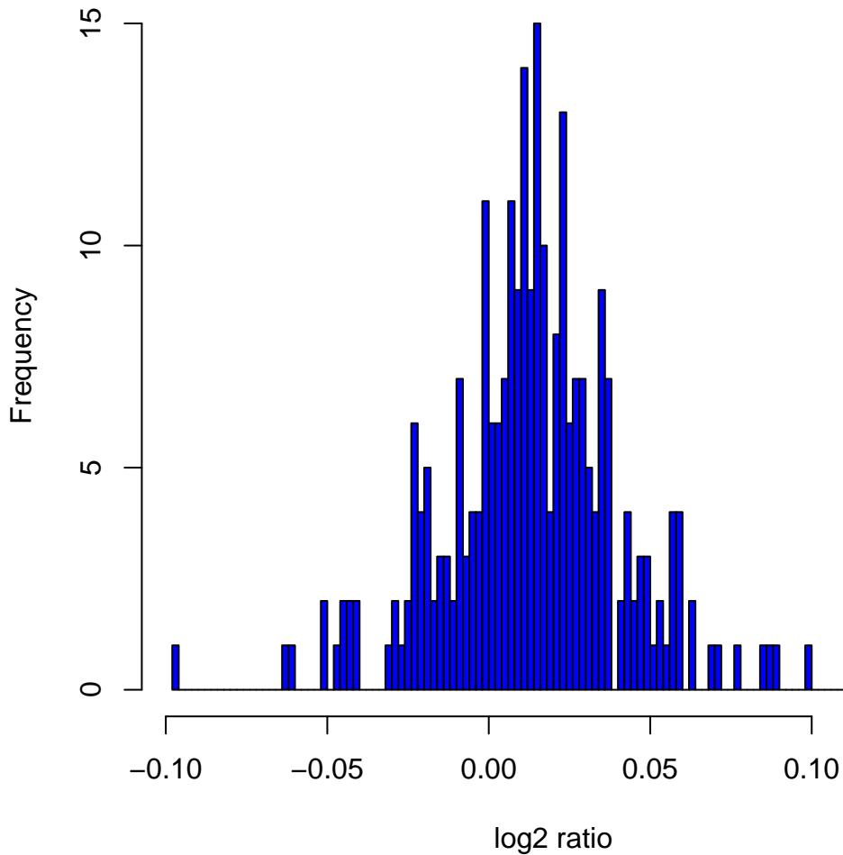
Histogram of log2ratios in 270 HapMap samples at clone Chr4tp-2E3
