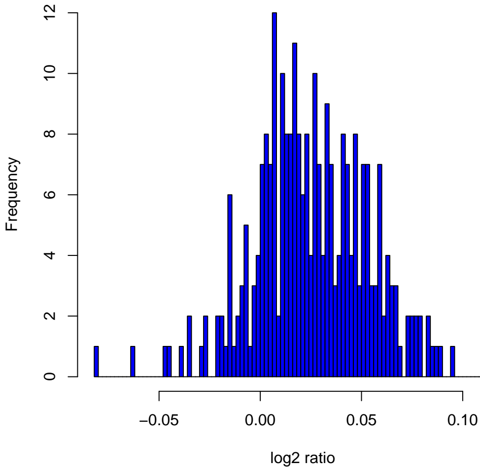
Histogram of \log_2 ratios in 270 HapMap samples at clone Chr4tp-2E4
