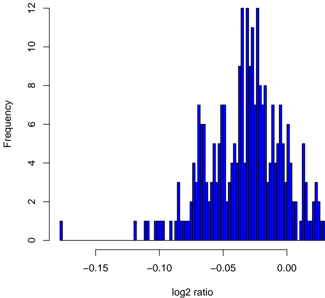
Histogram of log 2 ratios in 270 HapMap samples at clone Chr4tp-2H11
