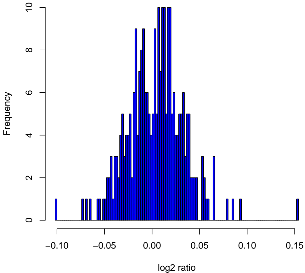
Histogram of log 2 ratios in 270 HapMap samples at clone Chr4tp-2H2
