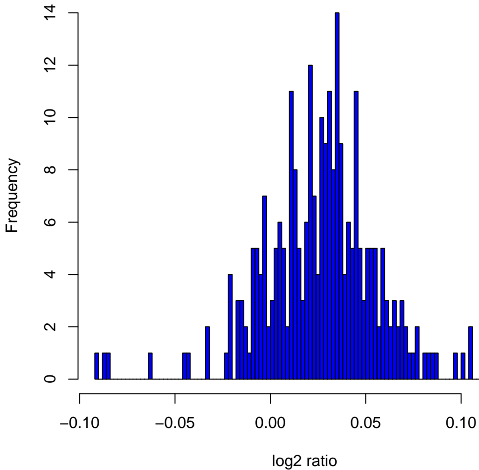
Histogram of log 2 ratios in 270 HapMap samples at clone Chr4tp-2H8
