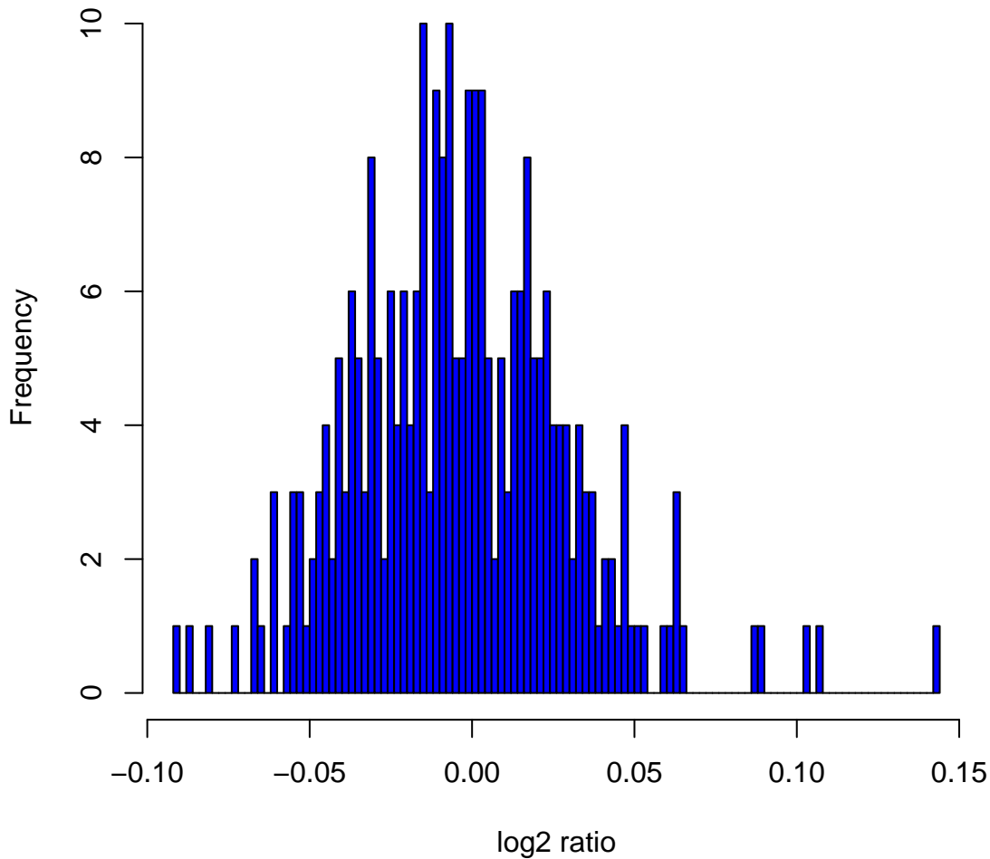
Histogram of log 2 ratios in 270 HapMap samples at clone Chr4tp-3A3
