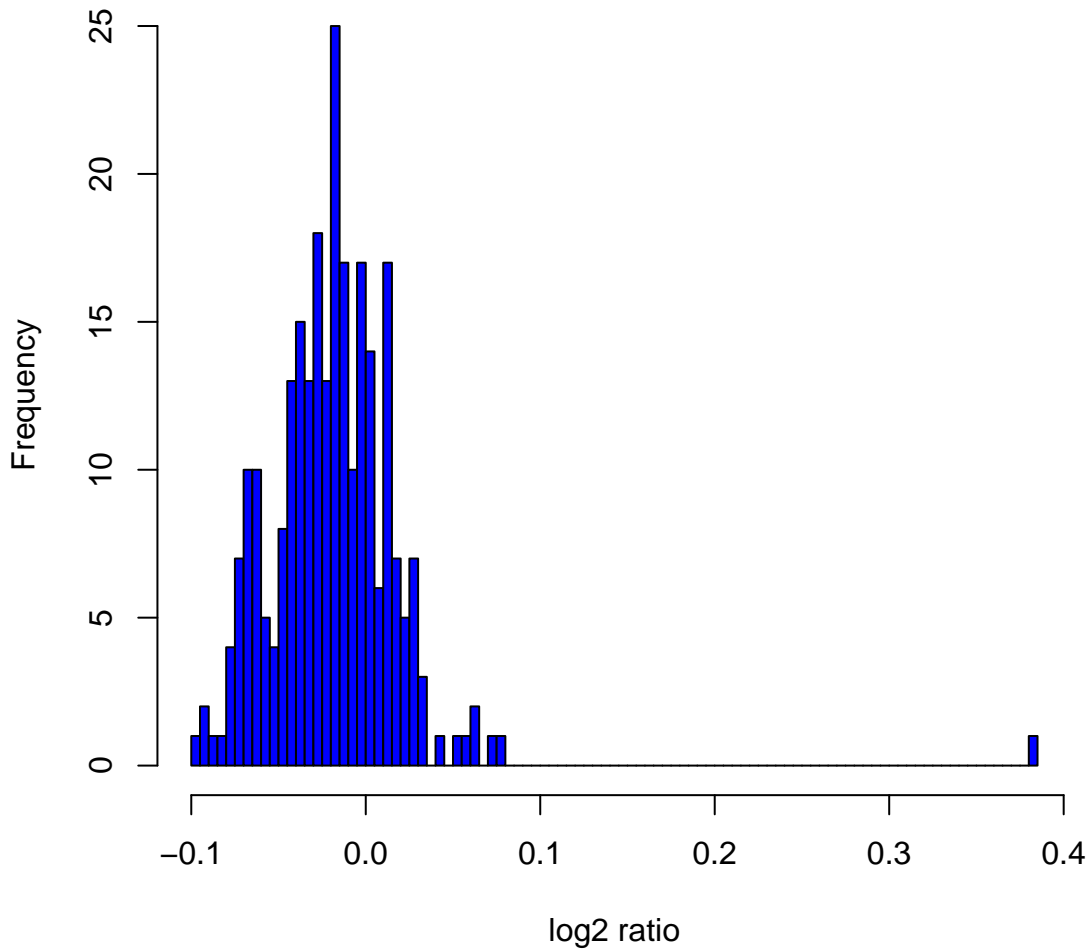
Histogram of log 2 ratios in 270 HapMap samples at clone Chr4tp-3B5
