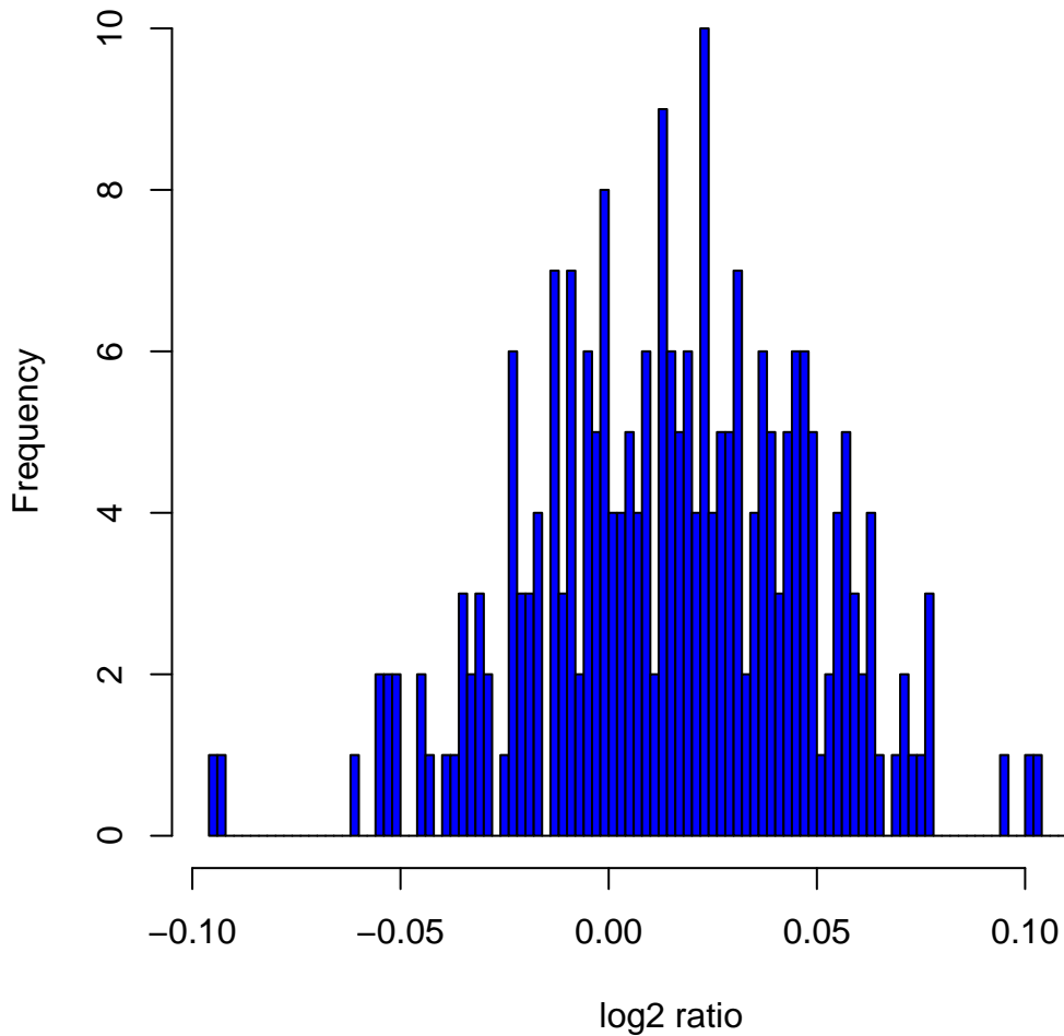
Histogram of \log_2 ratios in 270 HapMap samples at clone Chr4tp-3B7
