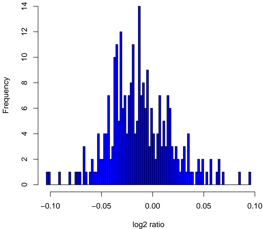
Histogram of log 2 ratios in 270 HapMap samples at clone Chr4tp-3C2
