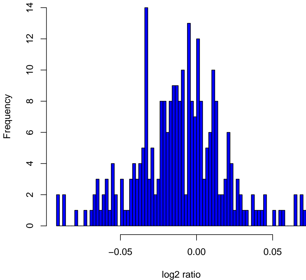
Histogram of log 2 ratios in 270 HapMap samples at clone Chr4tp-3D3
