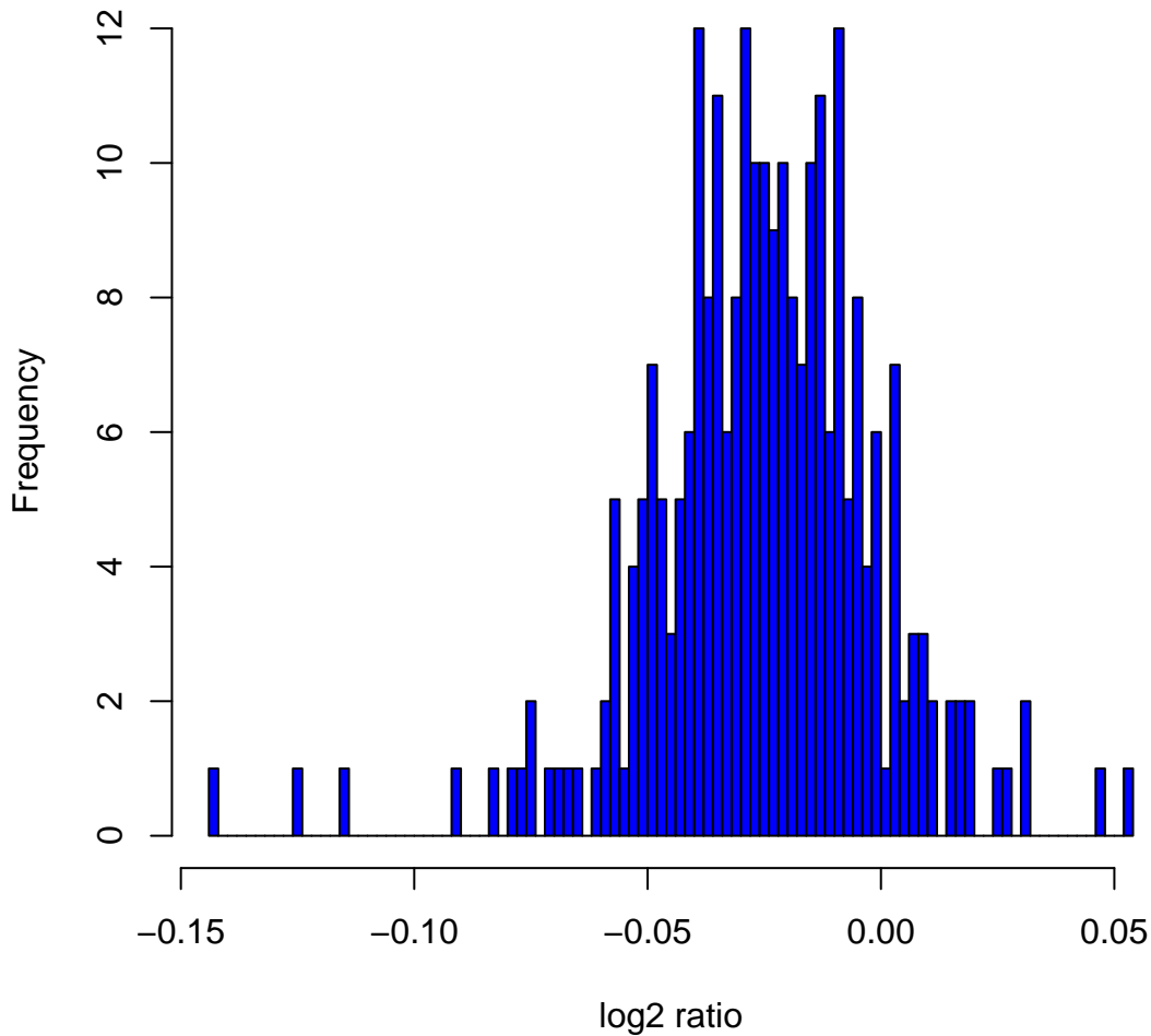
Histogram of \log_2 ratios in 270 HapMap samples at clone Chr4tp-3D4
