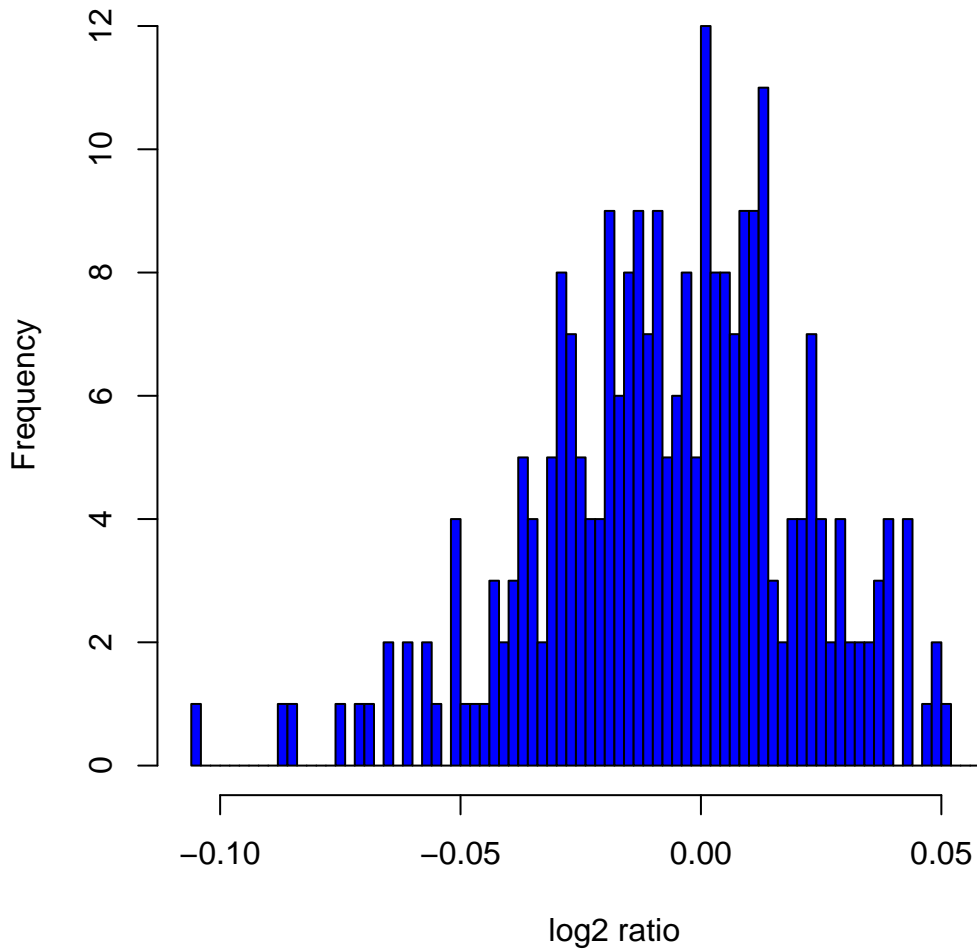
Histogram of \log_2 ratios in 270 HapMap samples at clone Chr4tp-3D8
