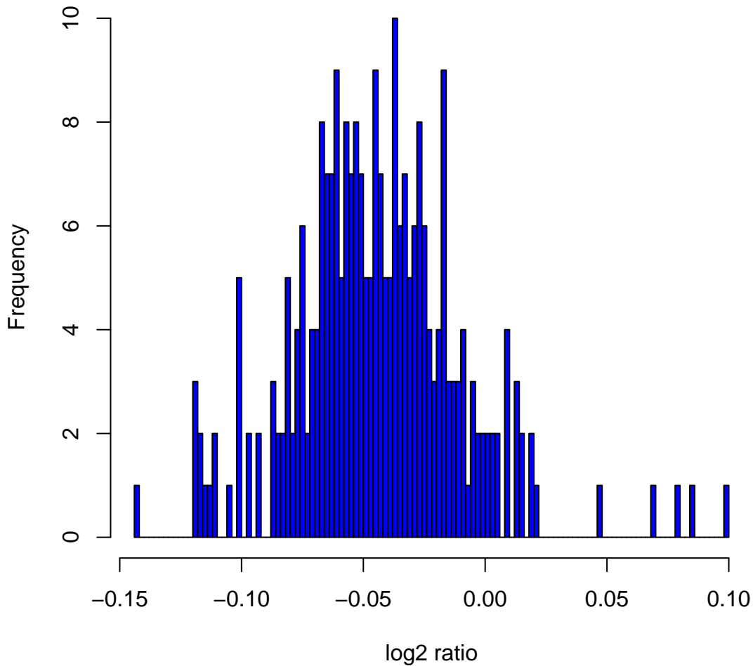
Histogram of log 2 ratios in 270 HapMap samples at clone Chr4tp-3E3
