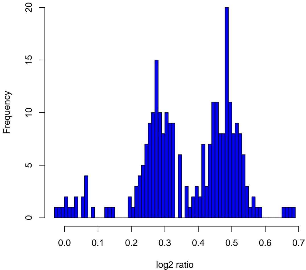
Histogram of \log_2 ratios in 270 HapMap samples at clone Chr4tp-3G3
