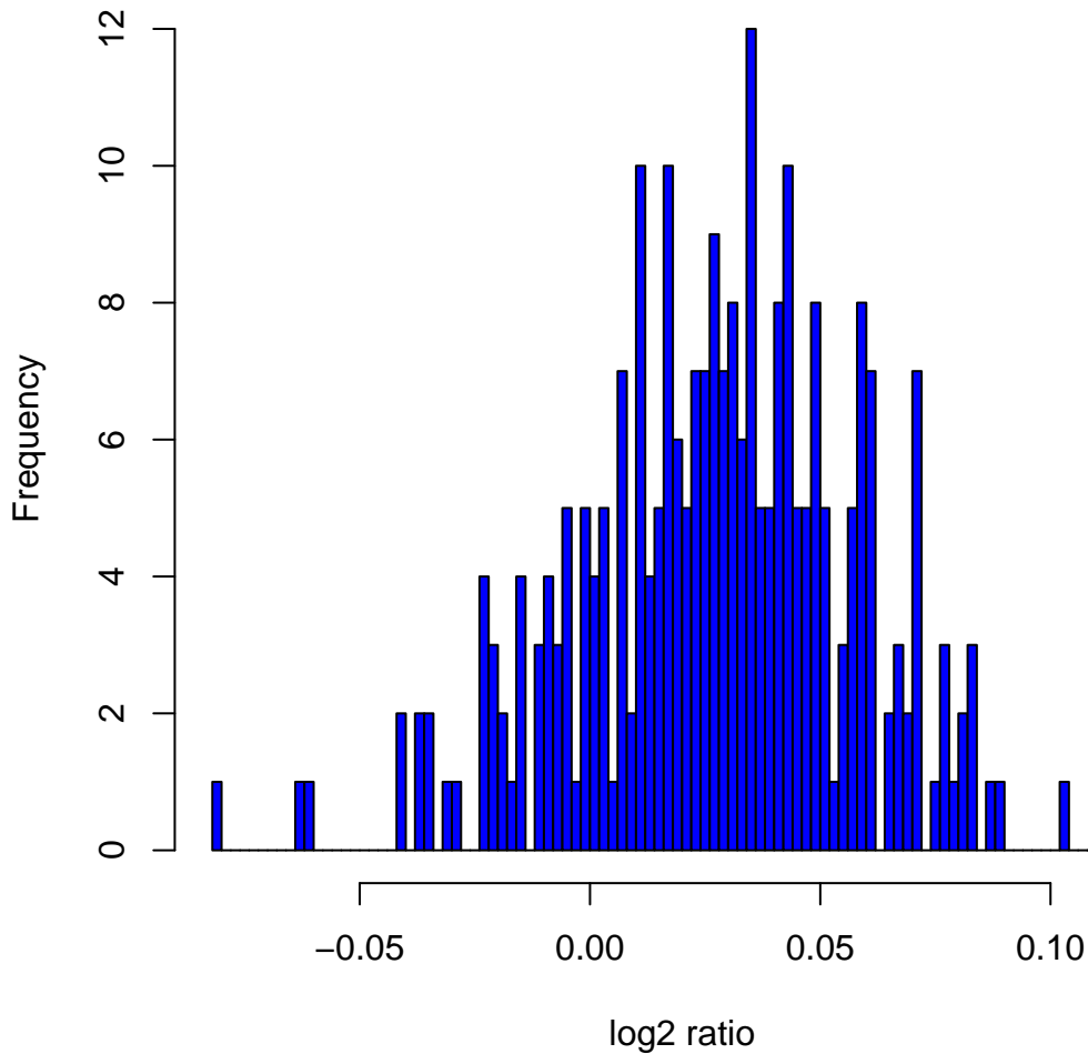
Histogram of log 2 ratios in 270 HapMap samples at clone Chr4tp-3G6
