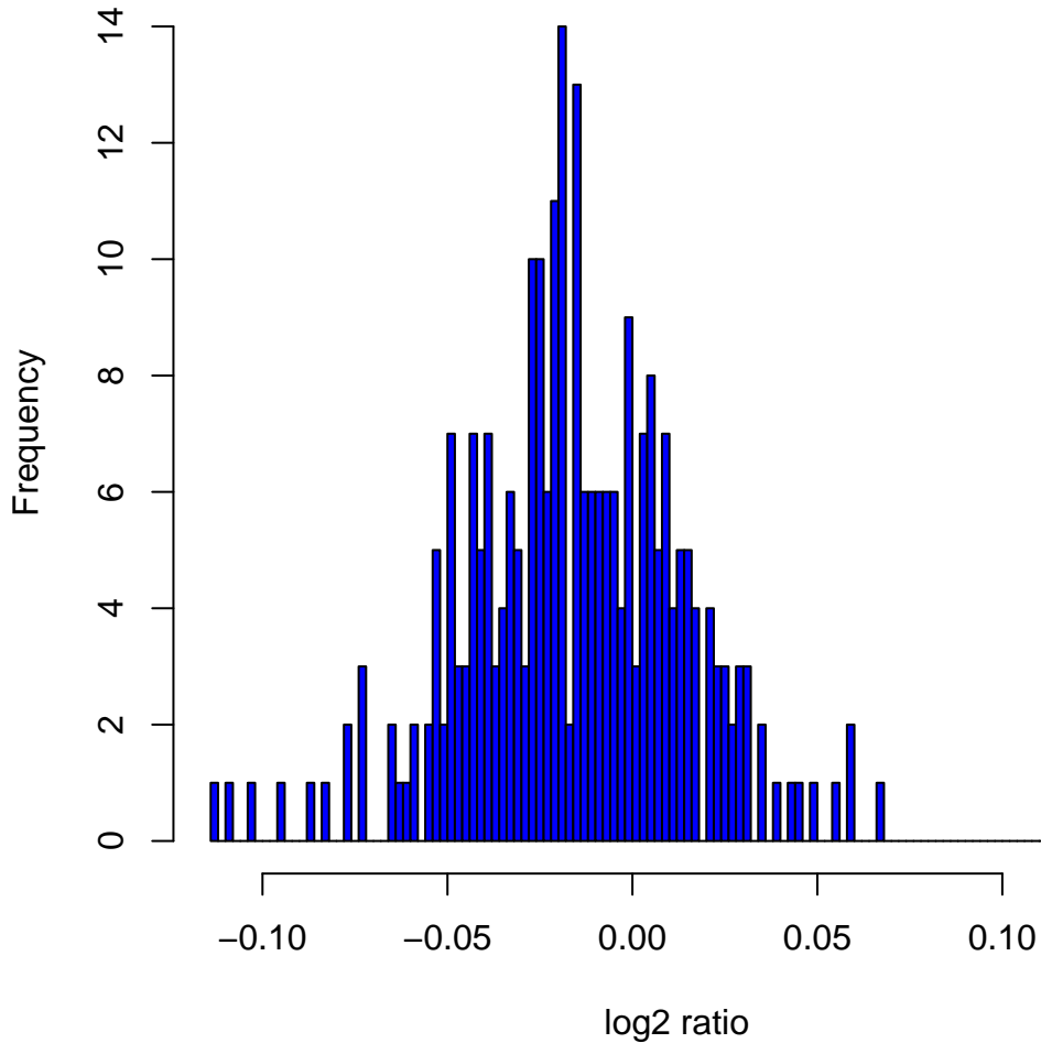
Histogram of log 2 ratios in 270 HapMap samples at clone Chr4tp-3H12
