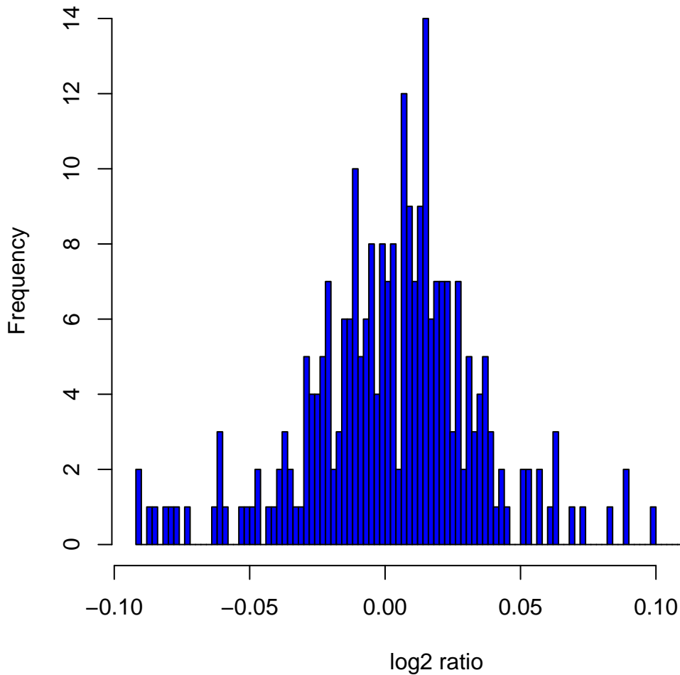
Histogram of log 2 ratios in 270 HapMap samples at clone Chr4tp-3H9
