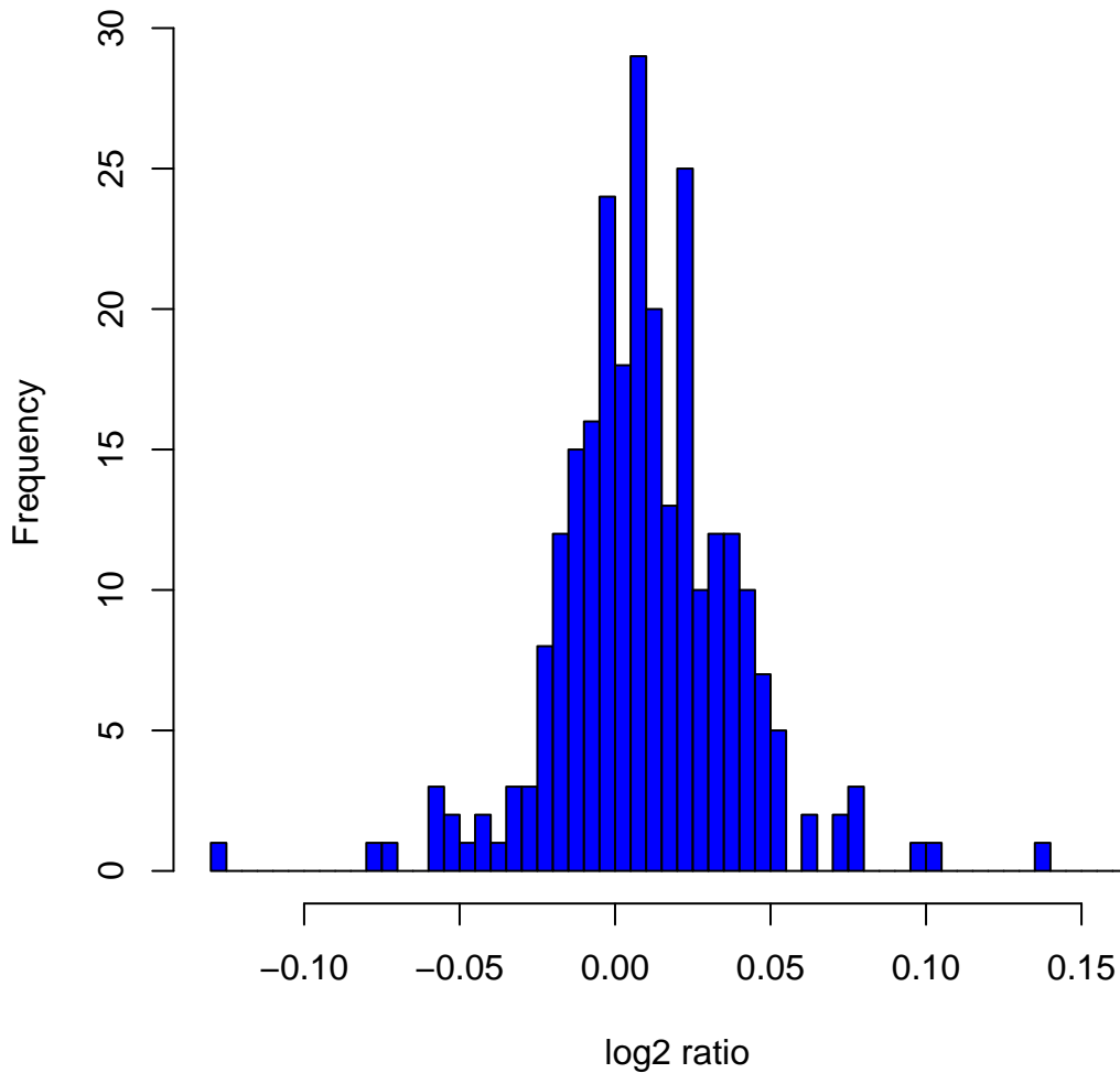
Histogram of \log_2 ratios in 270 HapMap samples at clone Chr4tp-4A8
