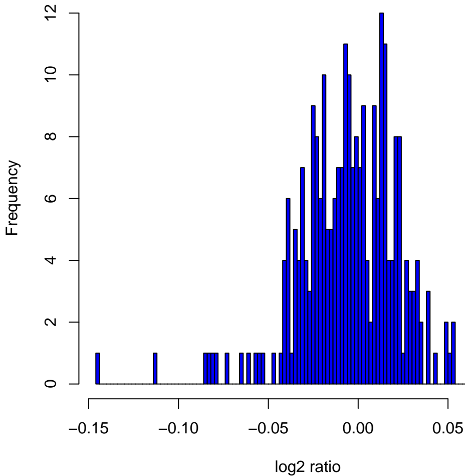
Histogram of log 2 ratios in 270 HapMap samples at clone Chr4tp-4C8
